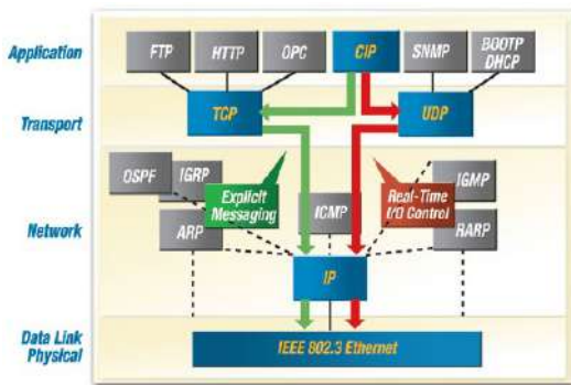
Figura 72 – Arquitetura Explicit e Implicit Messaging “Ethernet/IP™ Quick Start for Vendors Handbook (PUB213R0) ODVA”
